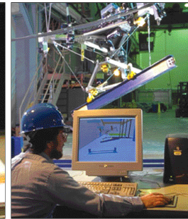
▲ NIST RoboCrane.
